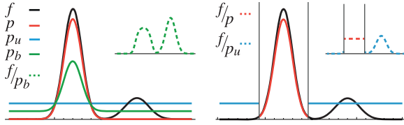
Figure 4: Left: The balance heuristic mixture p_b ruins the local proportionality of the aggressive distribution p to f by averaging it with the defensive uniform distribution p_u , while still resulting in lower than optimal probabilities outside the peak. Right: By adaptively partitioning the domain, the novel \alpha -max heuristic avoids mixing, selecting the distribution with closest proportionality in a user-controlled way.
