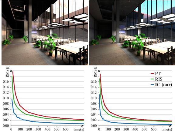
Figure 5: Top row: The STUDY HALL scene illuminated by 36 area lights and an environment map. Left: Direct illumination from St. Peter’s map. Right: Full global illumination from a sunset map. Bottom row: total image RMSE time convergence plots of path tracing (PT), resampled importance sampling (RIS) and importance caching (IC).
