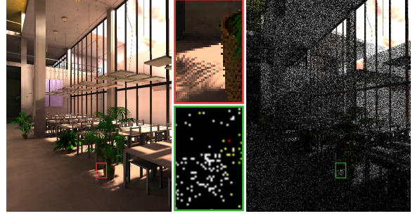
Figure 1: A scene illuminated by an environment map, with radiance field approximated by 6000 VPLs. Using only one VPL per pixel, chosen from a distribution proportional to its actual contribution, would result in perfect importance sampling, giving the exact solution (left). Excluding visibility from the distribution leads to excessive variance (right).
