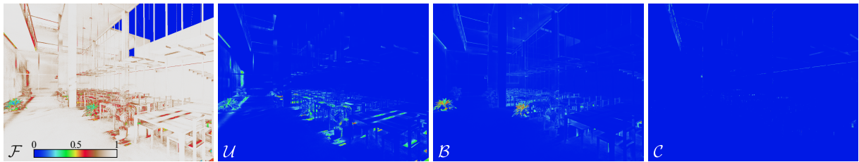
Figure 8: Fractional contributions of the sampling distributions used for the reference image in Figure 7. With the so chosen \alpha -max parameters, F captures 93.8% of the illumination, U and B account for 3% each, leaving 0.2% of the contribution to C .
