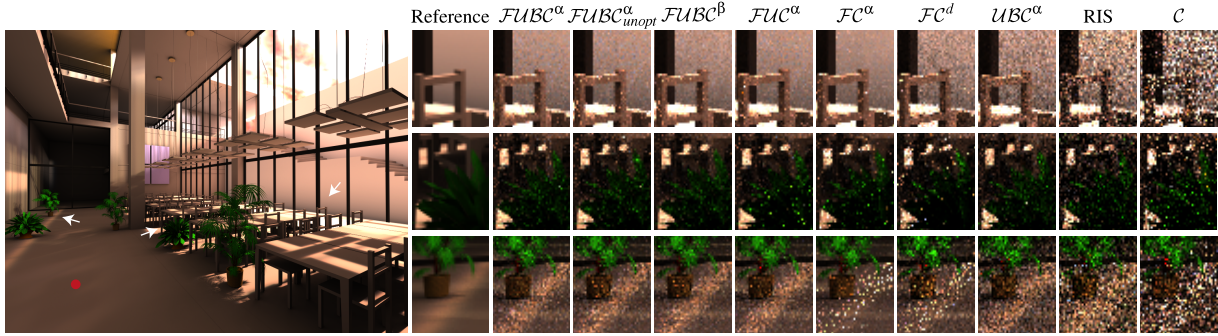
Figure 7: A comparison of different rendering setups. The label on each image denotes the techniques used for sampling and combination (as superscript). Each image uses 35 samples per pixel per frame, distributed manually among the sampling distributions to achieve the best result. The reference image was rendered using FUBC^\alpha in 1000s, the other images took 20s.
