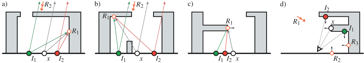
Figure 2: Four illumination conditions, encountered when reusing information from importance records (IRs) I_1 and I_2 at shading point x . At each IR we define four distributions, designed to discover VPL contributions under a different condition. a) In the case of smooth illumination in the local neighborhood, full contribution sampling ( \mathcal{F} ) can achieve close proportionality to the integrand. b) Unoccluded contribution sampling ( \mathcal{U} ) is robust to VPL contribution changes due to varying occlusion with position. c) Bounded contribution sampling ( \mathcal{B} ) in addition discovers new contributions due to orientation changes. d) Conservative uniform sampling ( \mathcal{C} ) handles situations where the IR importance information is irrelevant at the shading point x .
