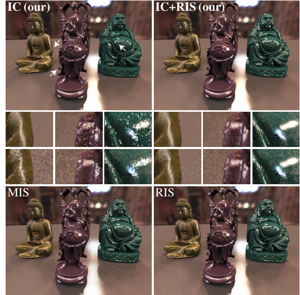
Figure 6: Glossy Buddha statues with Phong exponents, from left to right, 10, 80, 300 on a glossy ground with exponent 500, rendered in 20 sec using our importance caching algorithm (IC), resampled importance sampling (RIS), MIS-combined BRDF/illumination sampling (MIS), and combined IC and RIS (IC+RIS). In this worst case scenario for IC it still outperforms RIS and MIS in regions with occlusion and/or smooth illumination, while the combined IC+RIS algorithm achieves the best overall quality.
