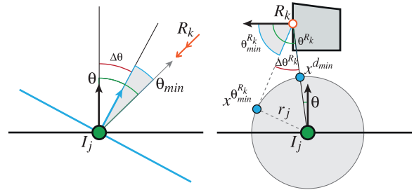
Figure 10: Bounding the geometric term in a neighborhood of record I_j for infinite (left) and finite (right) VPLs.
