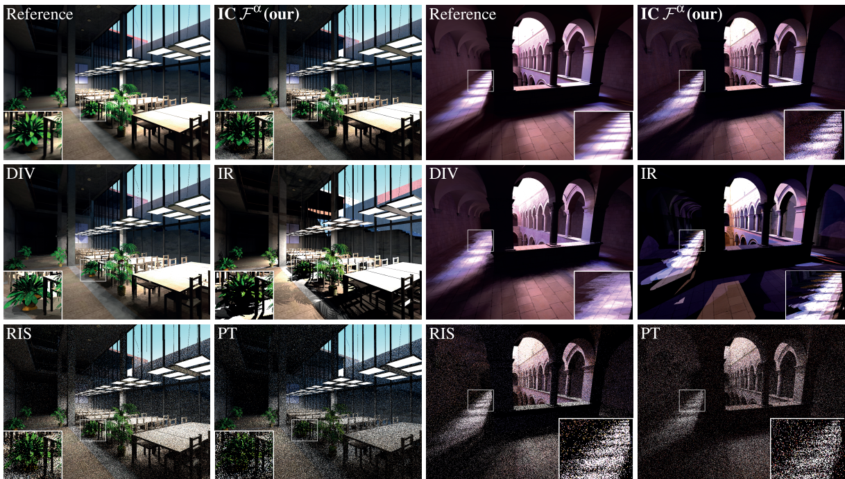
Figure 9: A 2-second full global illumination preview quality comparison on the STUDY HALL (left) and SPONZA (right) scenes between our importance caching algorithm using \alpha -max clamped F only ( IC F^\alpha ), direct importance visualization (DIV), instant radiosity (IR), resampled importance sampling (RIS) and path tracing (PT). Our algorithm ( IC F^\alpha ) produces a very low noise image close to the reference, and even without the U , B and C techniques handles well orientation and visibility discontinuities, which are blurred away by DIV. IR suffers from aliasing, while RIS and PT both produce very noisy results.
