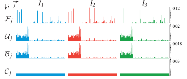
Figure 3: A matrix arrangement of the four distributions at the three closest records to the red-marked point in the left image in Figure 7. Notice the correlation among the columns. Direct illumination VPLs are in the beginning of the VPL list, hence the higher probabilities in the left.
